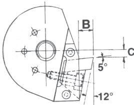
SHOWN WITH COOLANT ATTACHMENT
